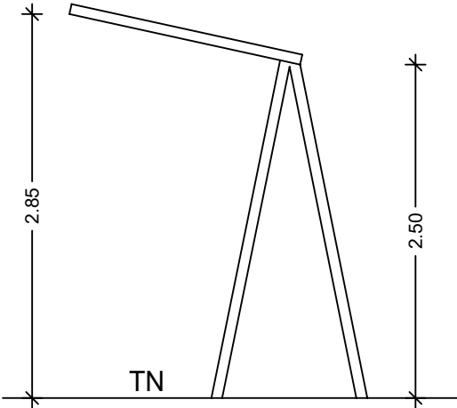
FACADE LATERALE
